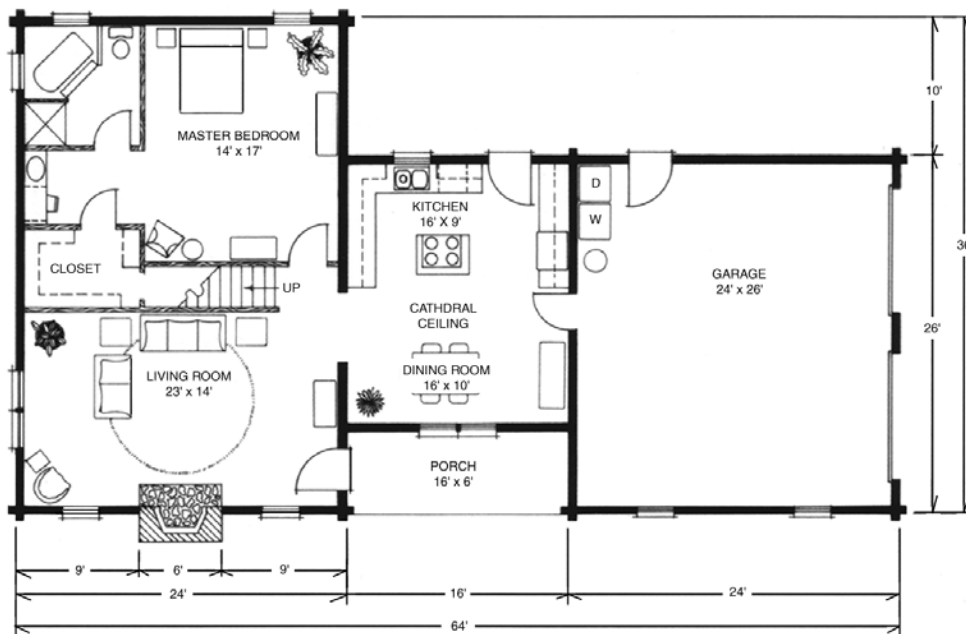
MAIN FLOOR
