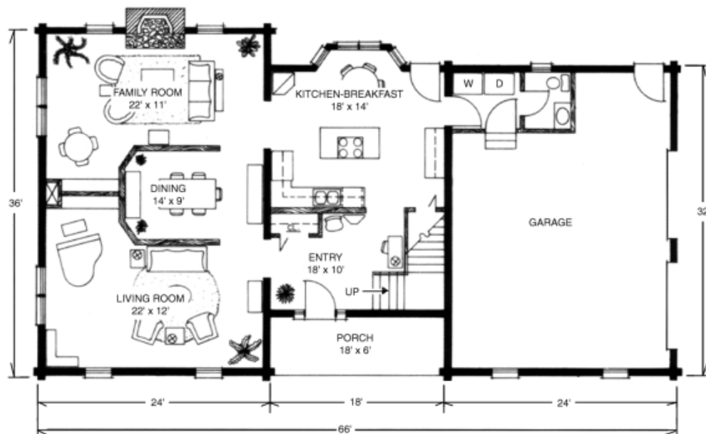
MAIN FLOOR
