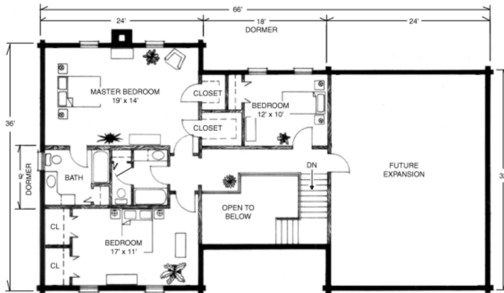
SECOND FLOOR
