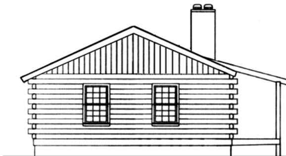
LEFT ELEVATION
